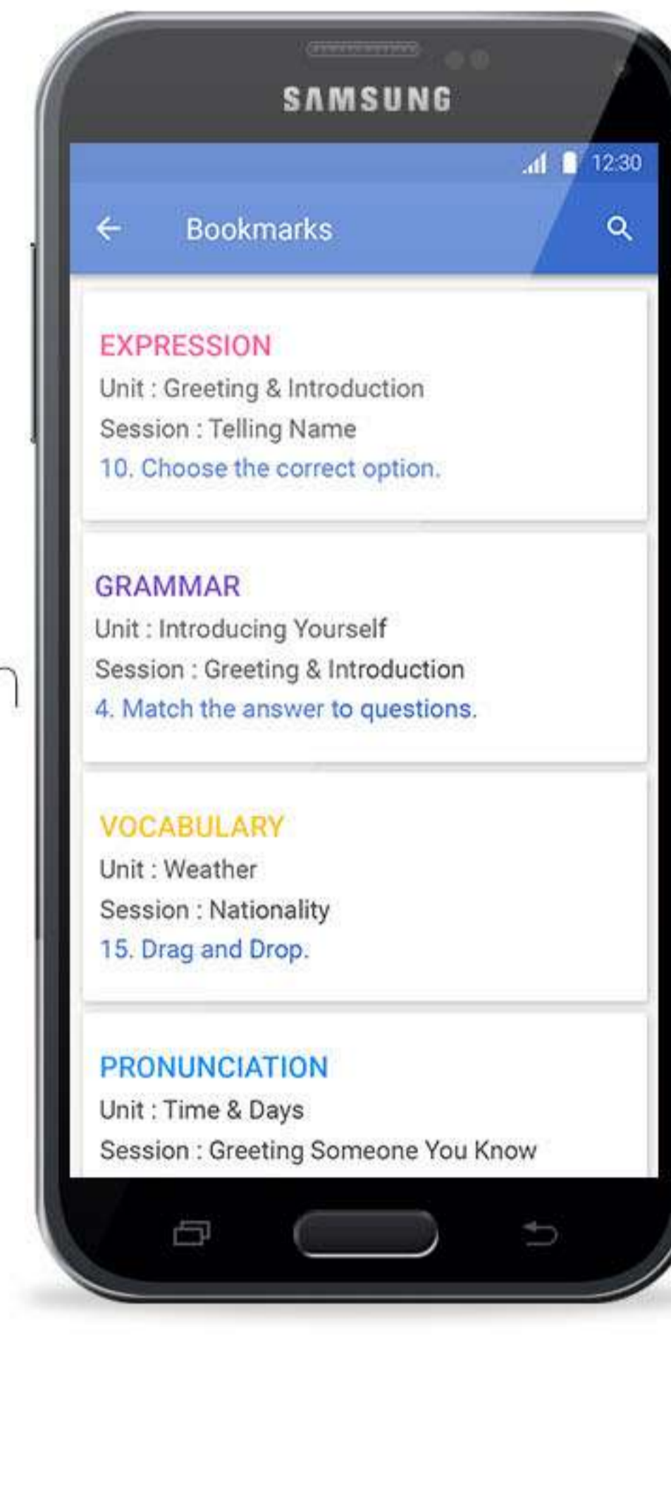
Bookmarks Screen
