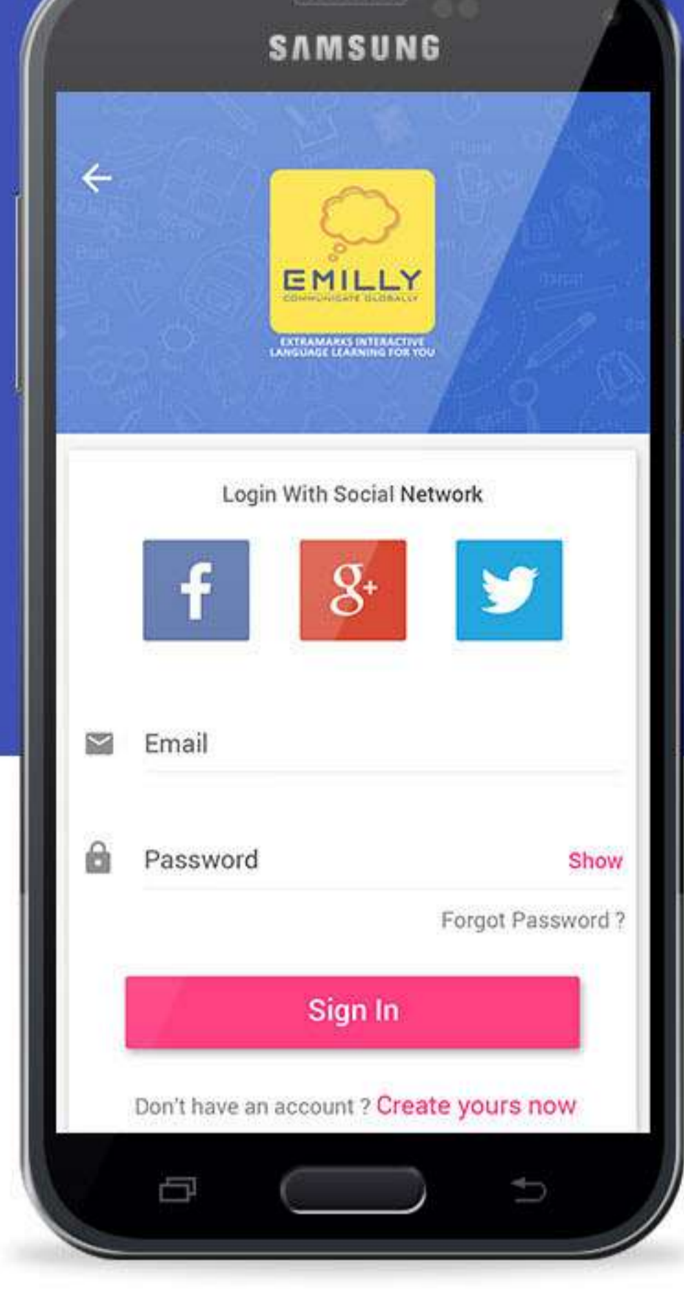
LogIn Screen
