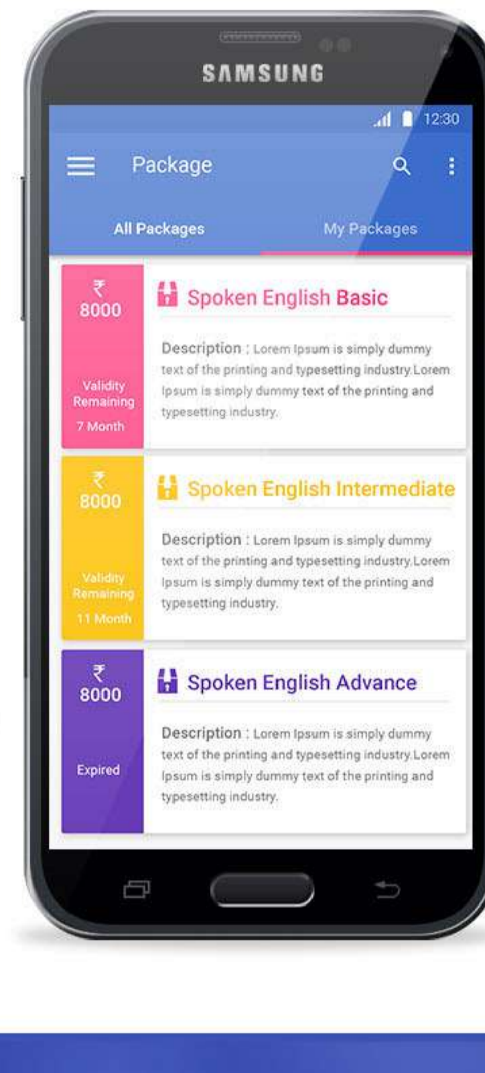
Package Screen
