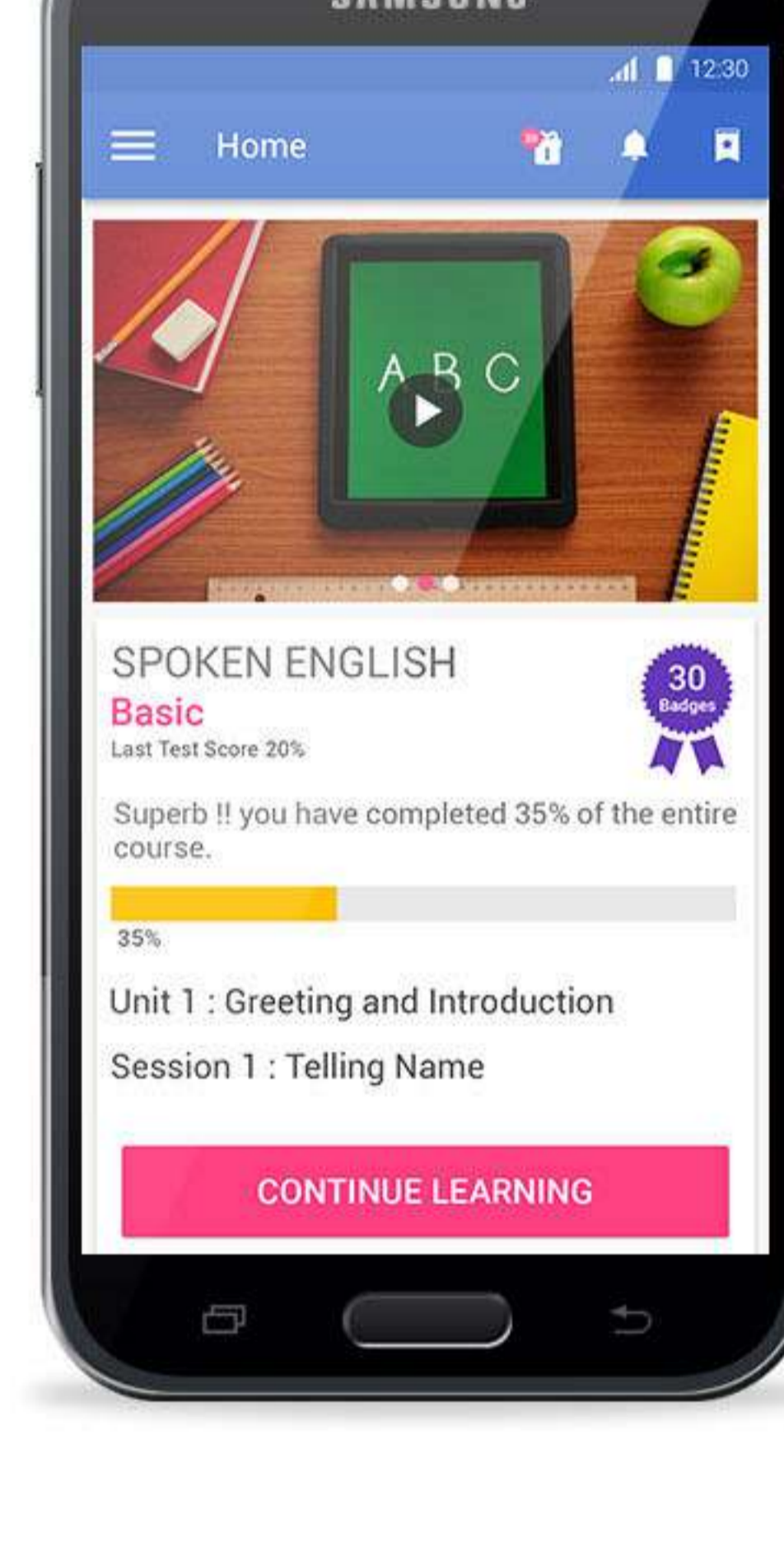
Home Screen
