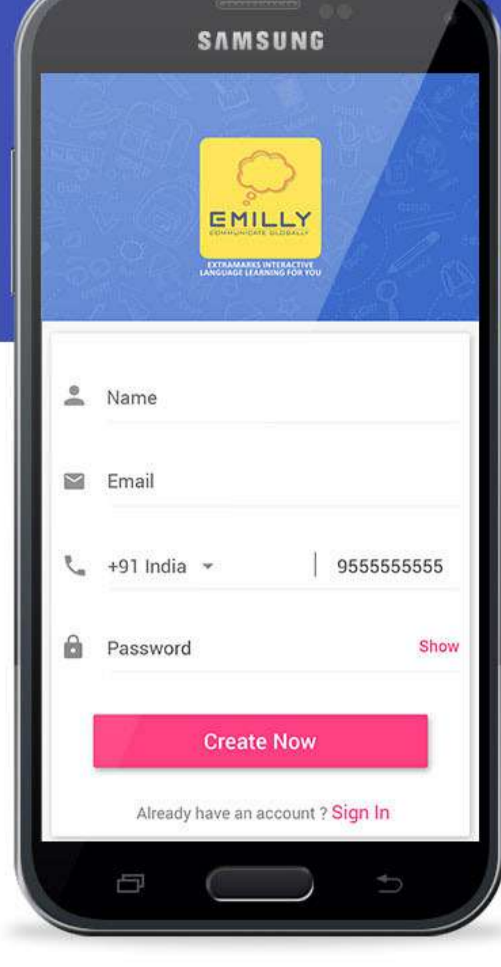
Signup Screen
