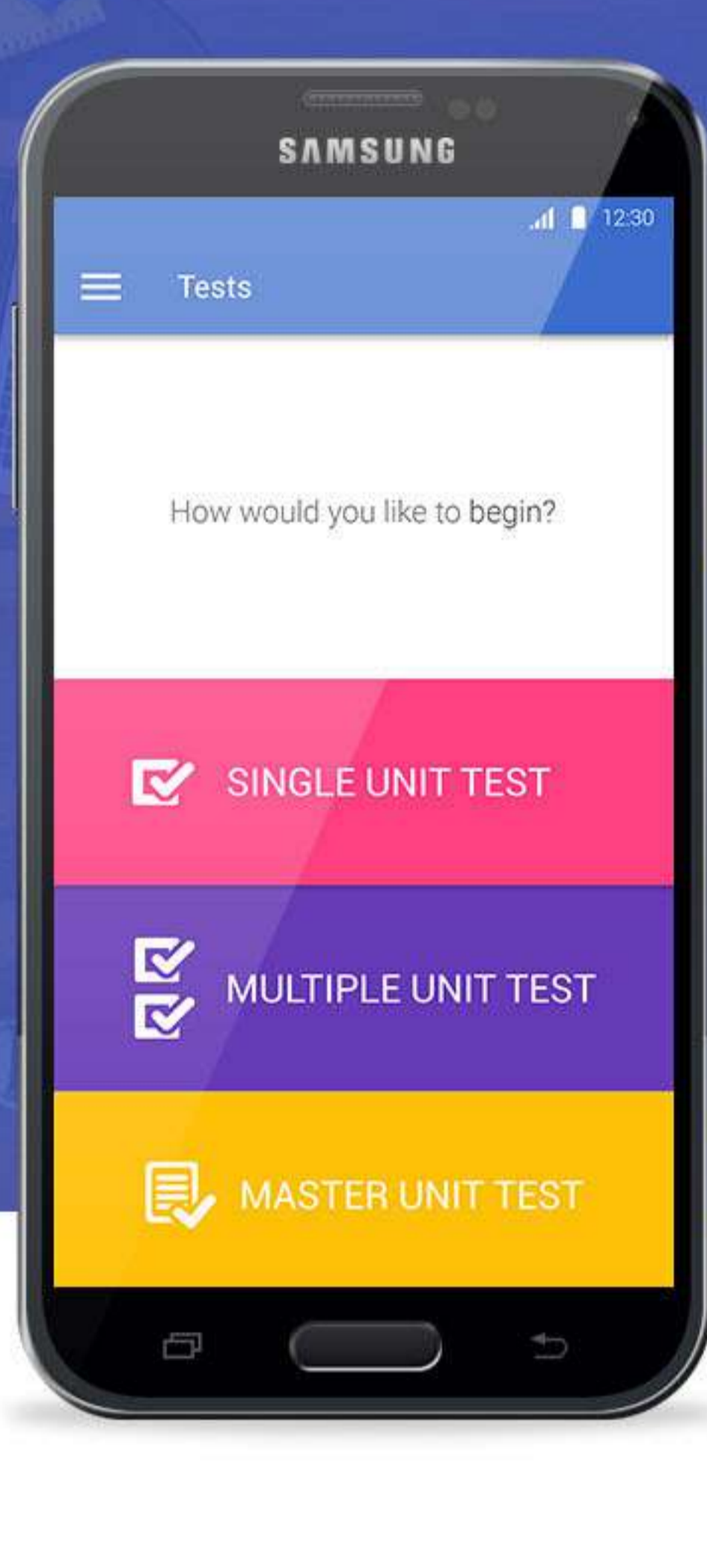
Select Test
