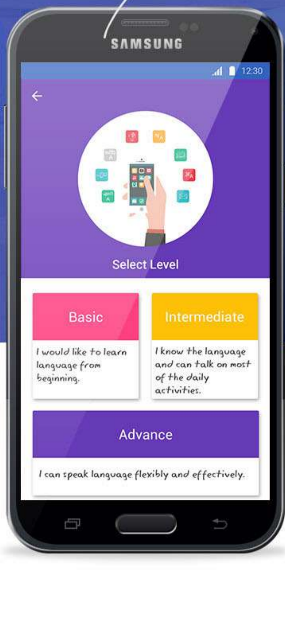
Select Level
